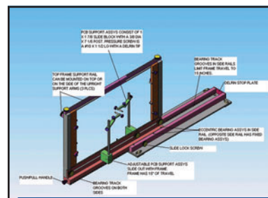
Vertically Mounted PCB System Applications
